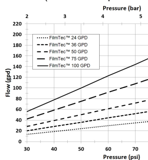
Figure 1: Impact of Pressure on Target Permeate Flow
